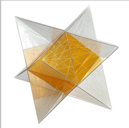
Stella octangula
