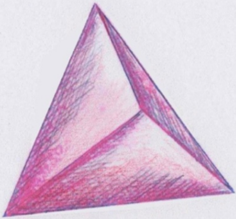
Tetraeder
