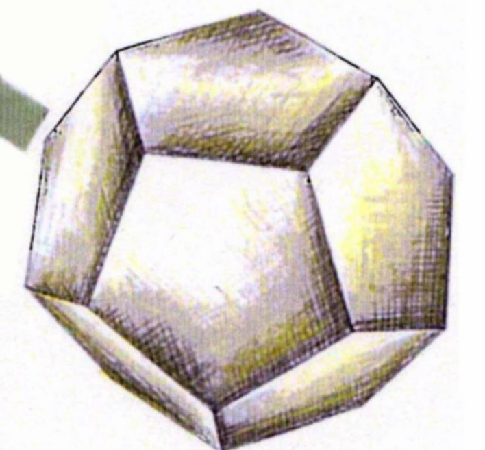
Pentagondodekaeder
